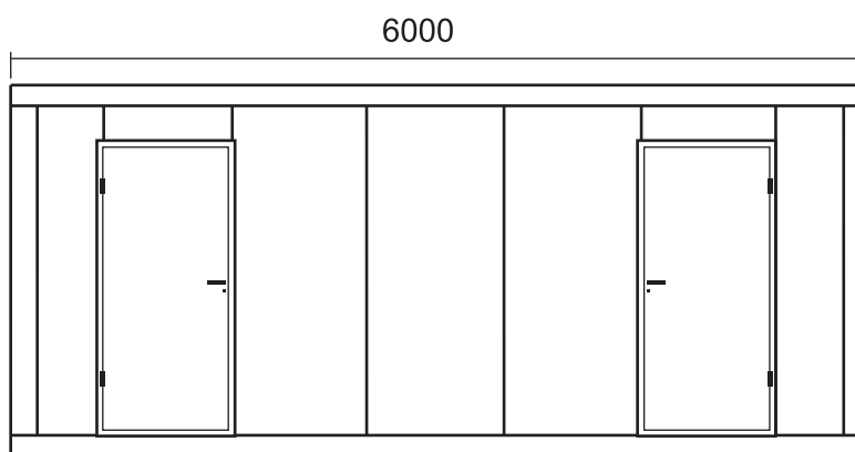
ALZADO PRINCIPAL
